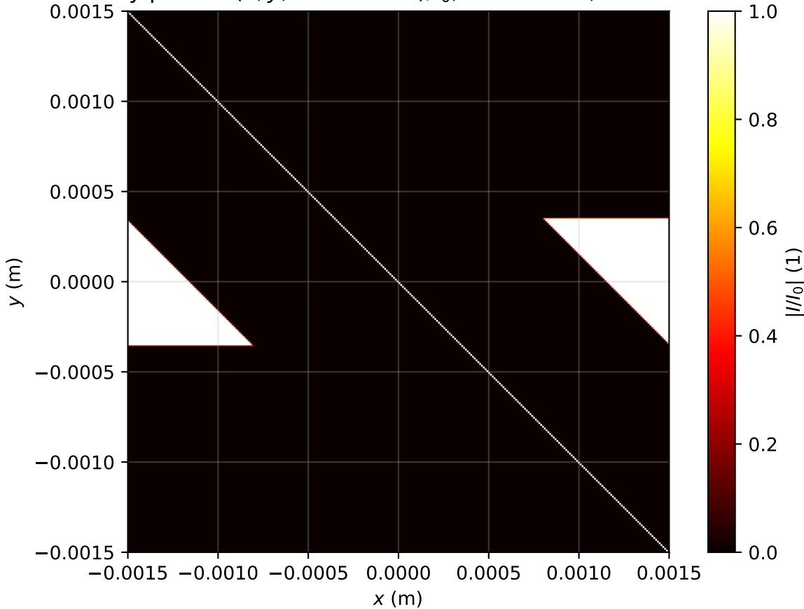
Intensity profile I(x, y, z = 0.000\text{m})/I_0 , P_{\text{in}}=4.0P_{\text{cr}} , artificial time
